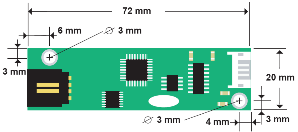
SE-E04R CONTROLLER
